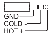
Fig3. JackBal Input / Output Pin-out
